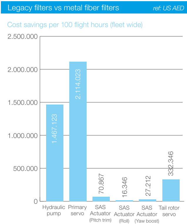
Figure 6. Cost savings achieved through the use of metal fiber filter media.
